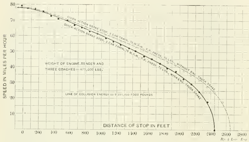
FIG. 2. RUN MADE TO DEMONSTRATE ADVANTAGE OF ENGINE TRUCK BRAKE Collision speed, 24 miles per hour. Collision energy, 9,891,000 foot pounds.
